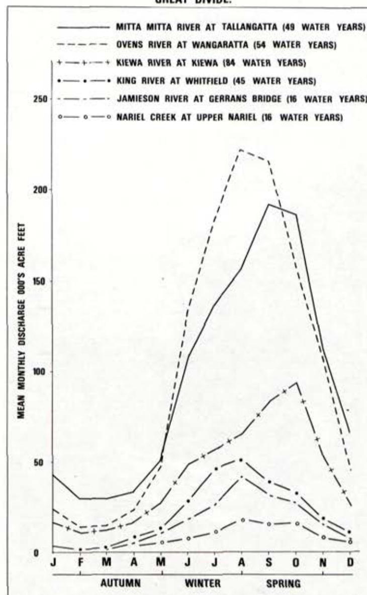
FIGURE 4 MEAN MONTHLY DISCHARGE-STREAMS NORTH OF GREAT DIVIDE.
