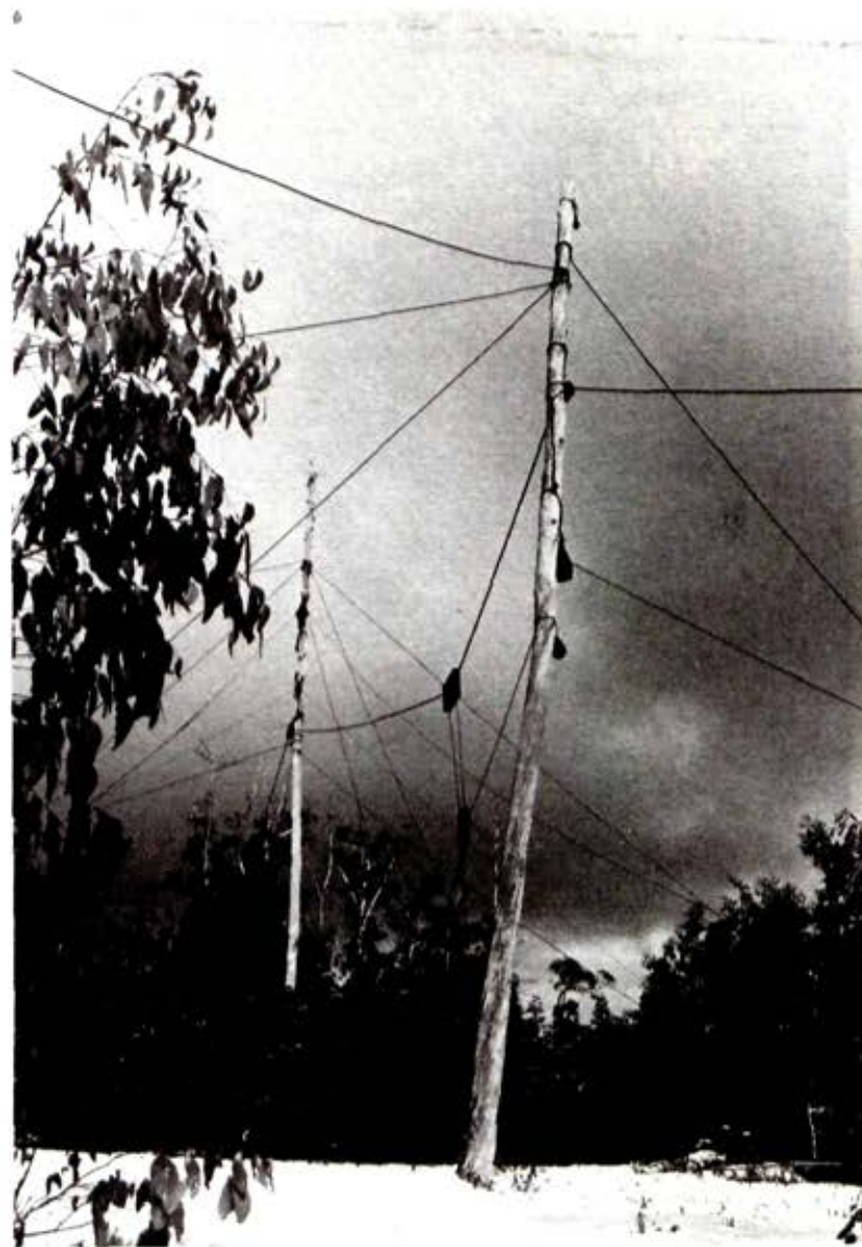
Spar trees, cables, and pulleys near Mount Nugong used for high-lead logging in the 1950s.
